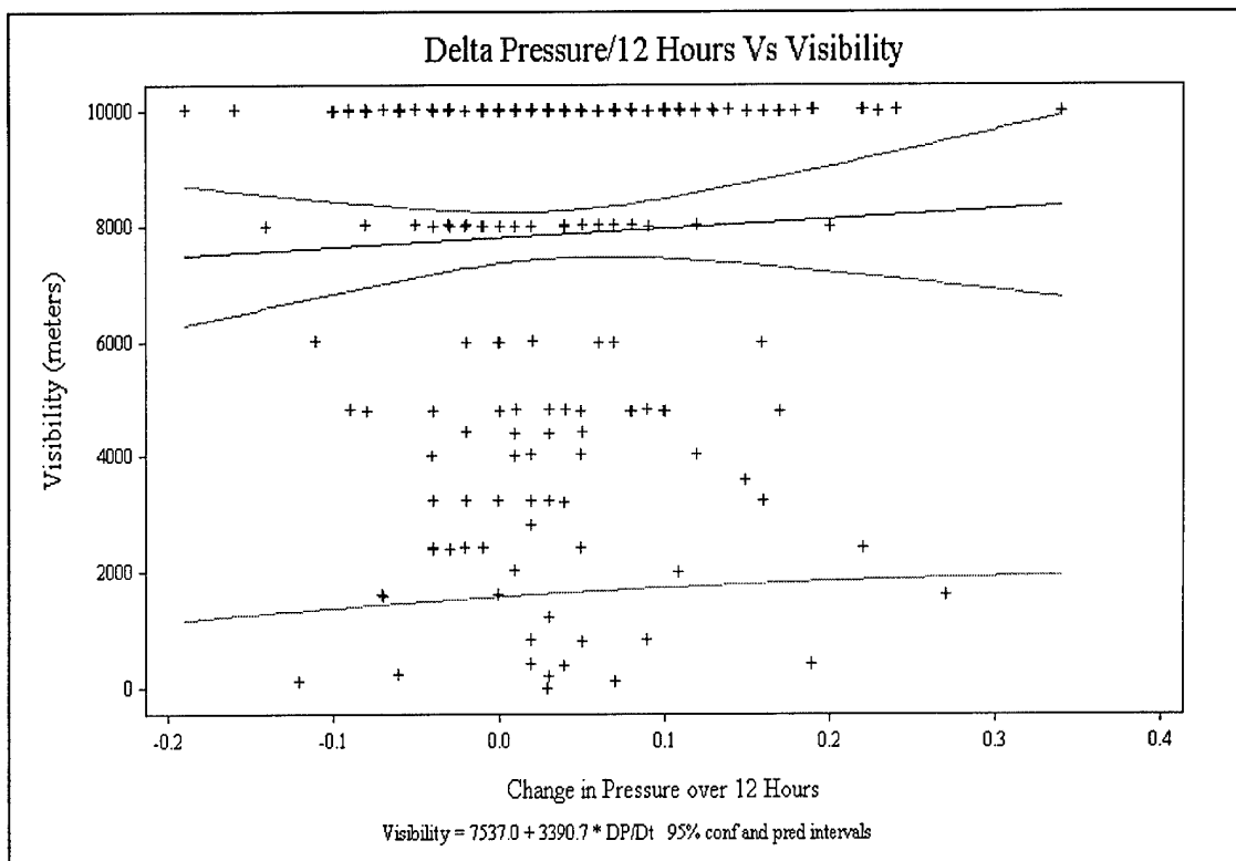
Figure 4.8. Delta Pressure/12 Hours Vs Visibility. The change in surface pressure (inches of mercury per 12 hours) was plotted versus the resulting visibility.
