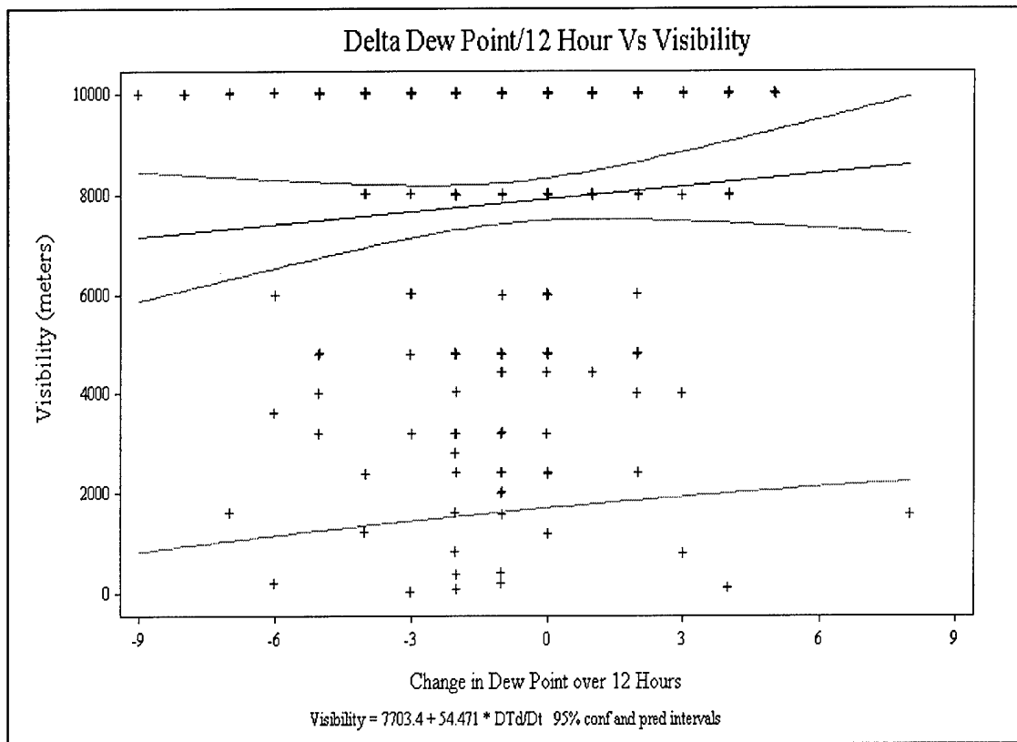
Figure 4.11. Delta Dew Point/12 hours Vs Visibility. Here the change in surface dew point over 12 hours was plotted versus the resulting visibility.
