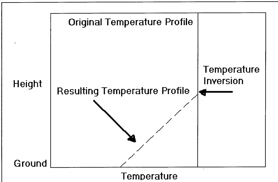
Figure 2.2. Cooling of the Near Surface Airmass. Resulting temperature profile indicates a temperature inversion has formed at the point where the change in temperature with height equals 0.0
